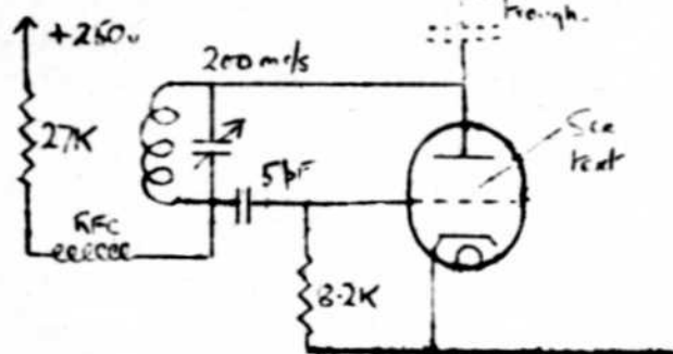
Fig ii. Circuit of 200 mc/s oscillator for unit.
